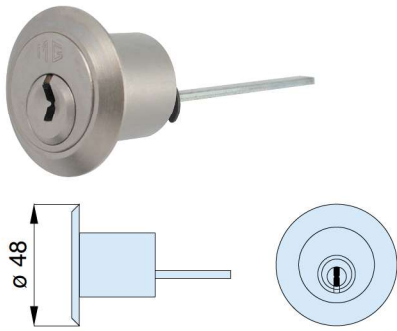
Cilindro per art. 712 Cylinder for art. 712
